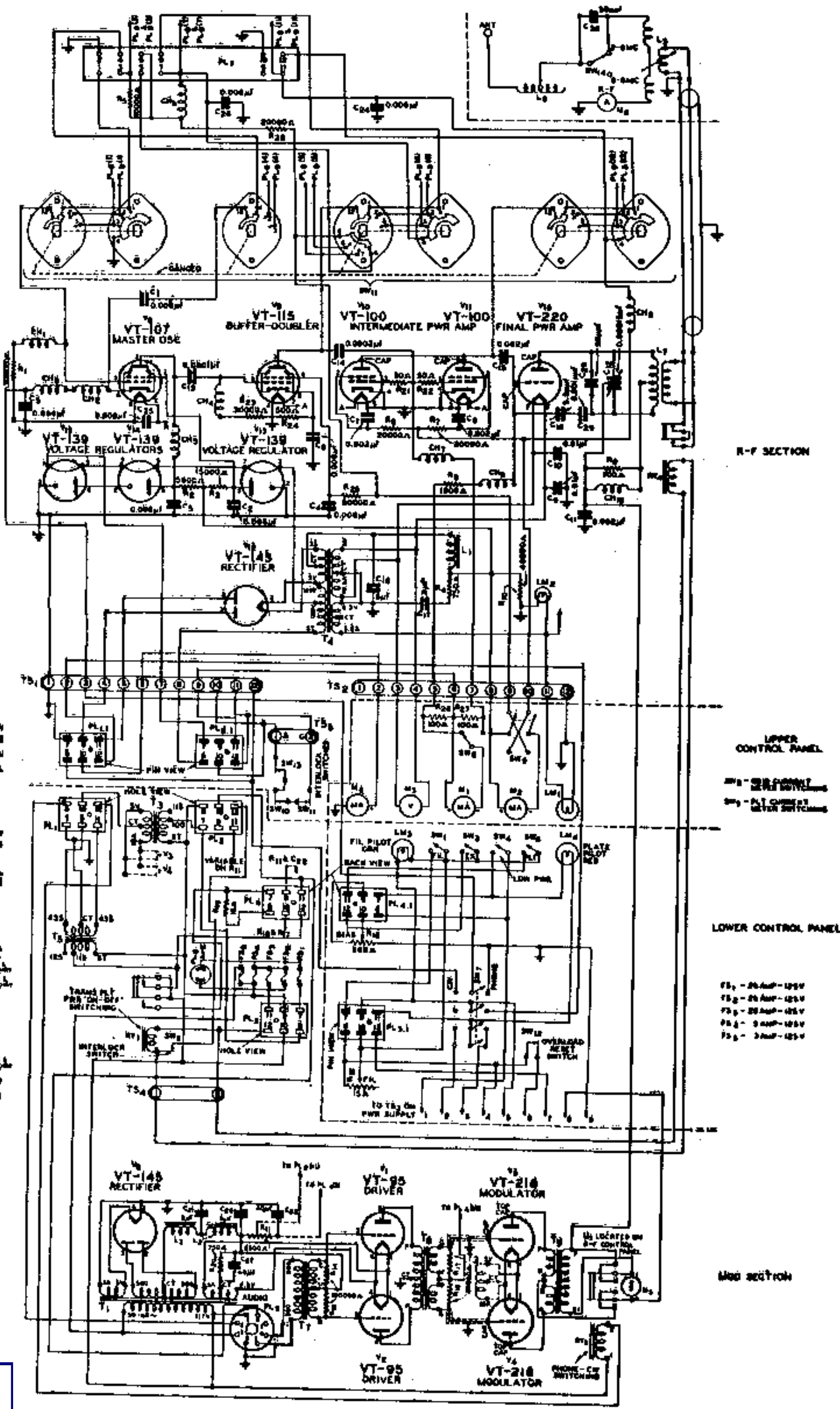
Fig. 8.—Schematic BC-610-C
